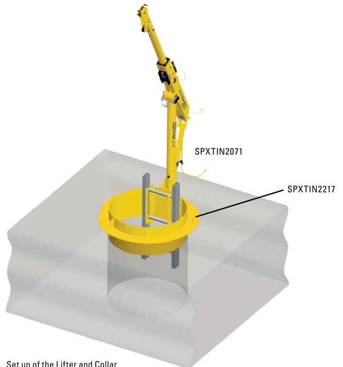
Set up of the Lifter and Collar
