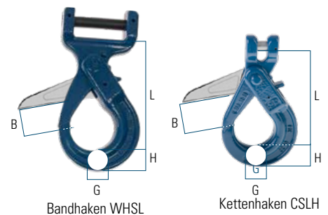
Bandhaken WHSL
