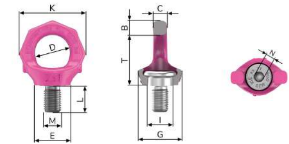
Golfari orientabili VRS StarPoint - GR100 - EN1677 - C.S. 4:1
