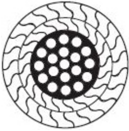
Locked Coil Strand
