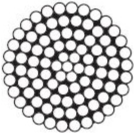
Spiral Strands
